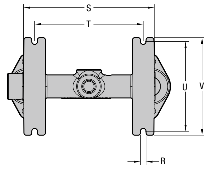
ALTERNATE FOOTPRINT
